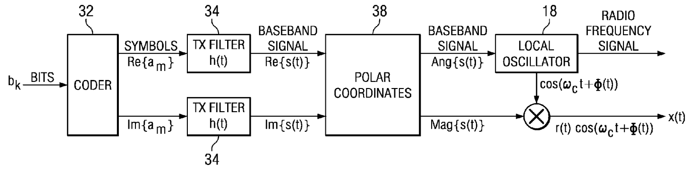
FIG. 4 (PRIOR ART)
